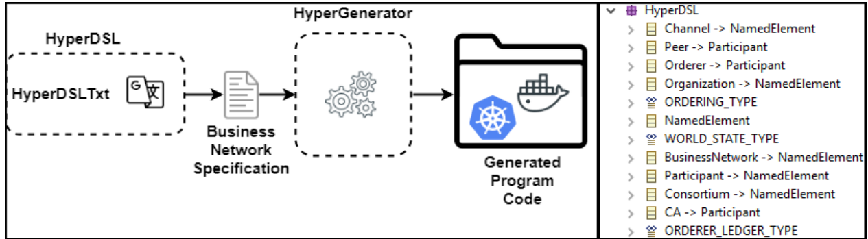
Figure 1. The HyperBuilder architecture and the HyperDSL meta-model
