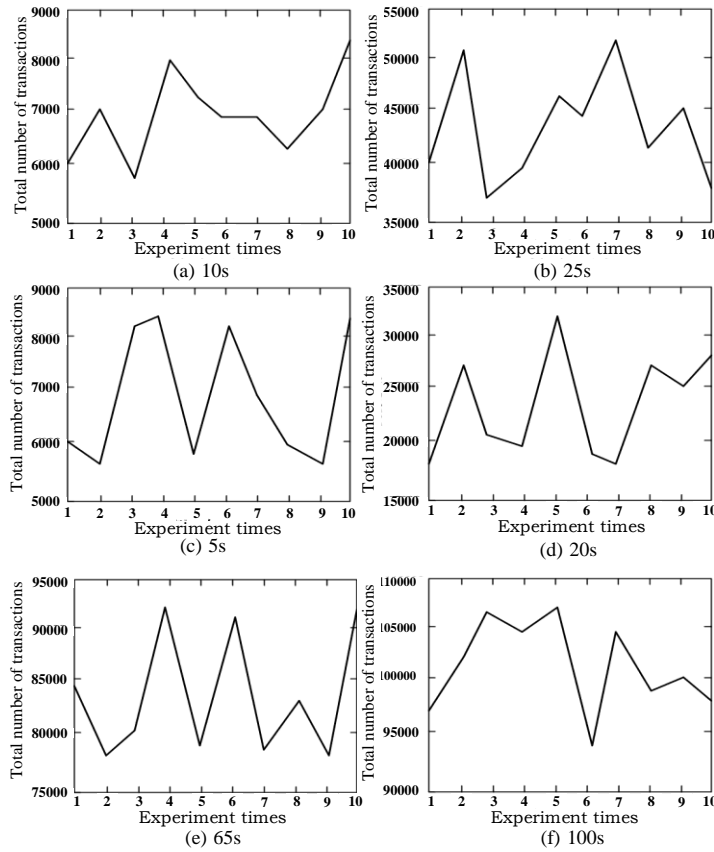
Figure 6. Change of total number of transactions when time interval changes
