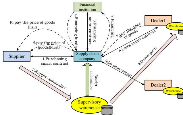
Figure 5. An intelligent contract model for procurement of goods in advance in the supply chain
