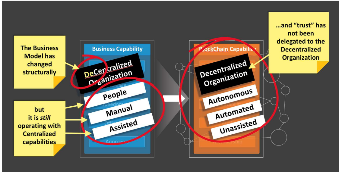
Figure 9: transformation - decentralized-to-decentralized
