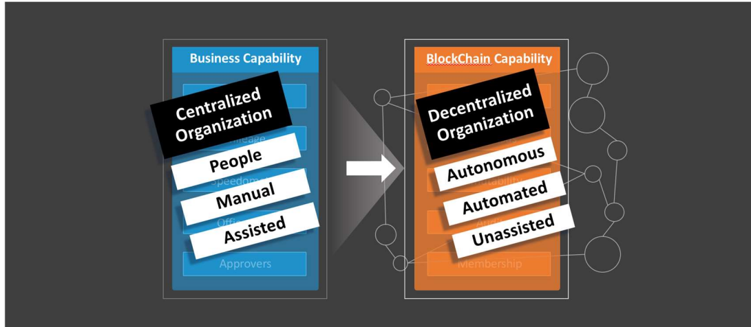
Figure 7: transformation - centralized-to-decentralized
